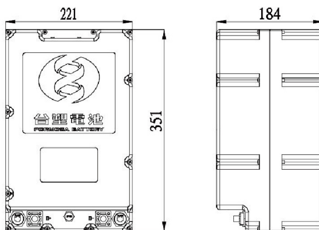
Fig. CONTROL BOX
