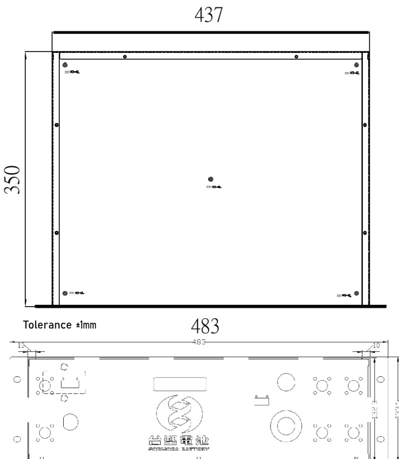
Fig. CONTROL BOX
